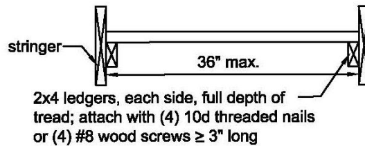
SOLID STRINGER
