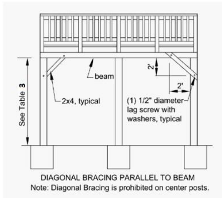
Figure 15. Diagonal Bracing
