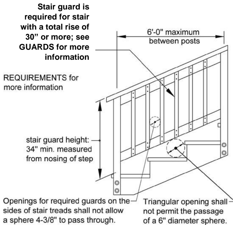
Figure 26. Stair Guard Requirements
