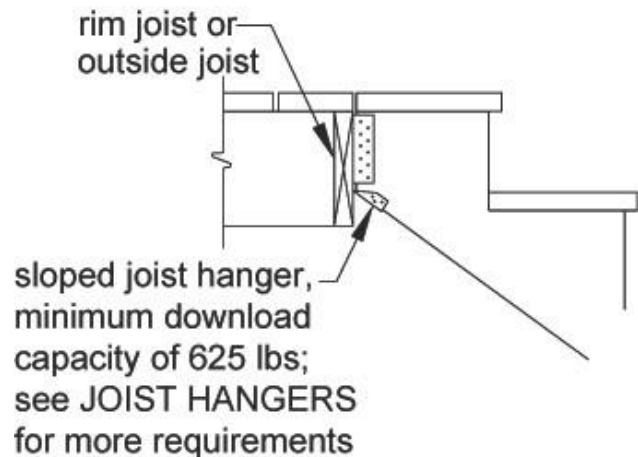
Figure 24. Stair Stringer Attachment Detail
