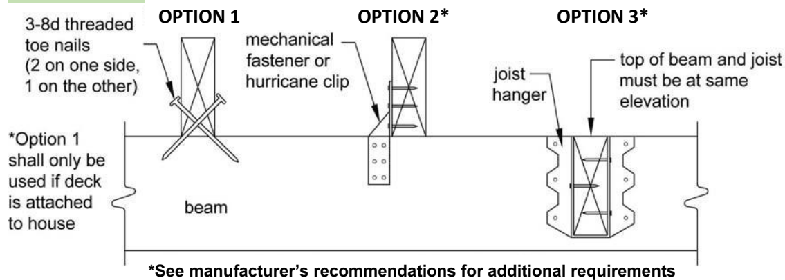
Figure 5. Joist-to-Beam Detail
